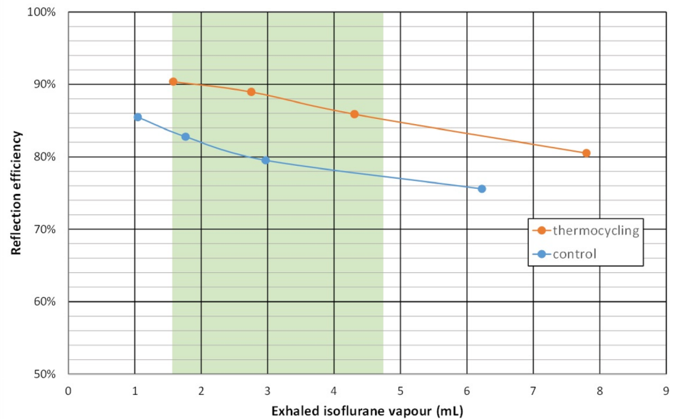
Fig. 3 Reflection efficiency during thermocycling and under control conditions plotted over the isoflurane vapor volume expired in one breath. In clinical practice, most commonly between 1.6 mL (e.g., tidal volume 400 mL, isoflurane concentration 0.4 Vol%) and 4.8 mL (tidal volume 800 mL, isoflurane concentration 0.6 Vol%) isoflurane vapour will be exhaled (green area)
