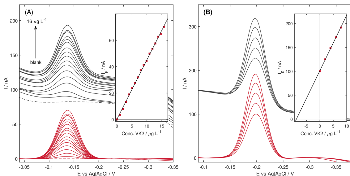
Fig. 4 A DP AdSV voltammograms recorded at CGMDE for concentrations of vitamin K 2 in the range from blank to 16 µg L -1 . B Determination of VK 2 produced by Bacillus subtilis bacteria after 240 h of breeding. Inset: corresponding calibration plots. Gray lines represent
