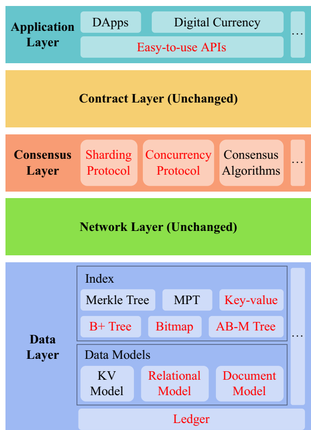
Fig. 3 Architecture of database-oriented blockchains
